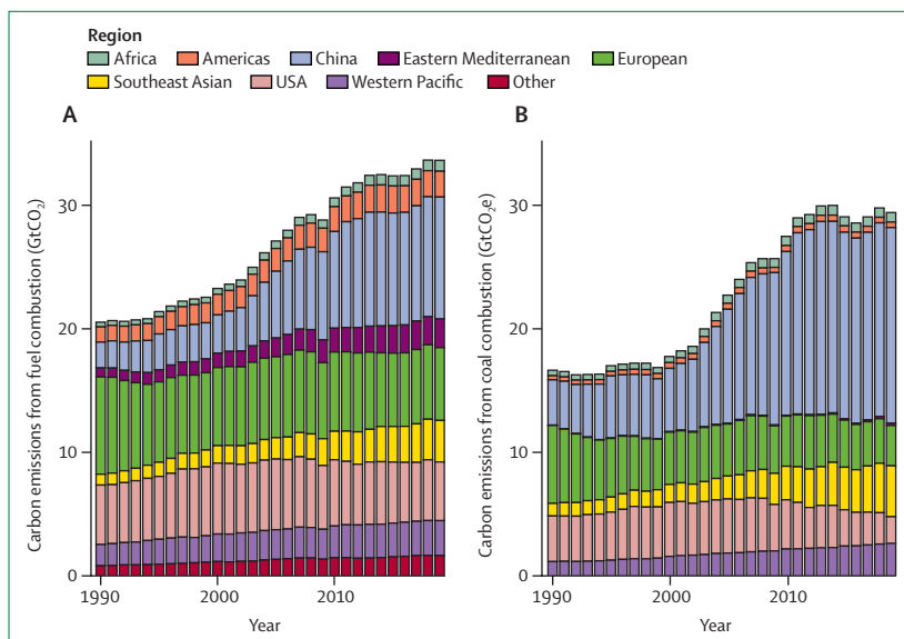
Figure 7: Greenhouse gas emissions from the global energy system
